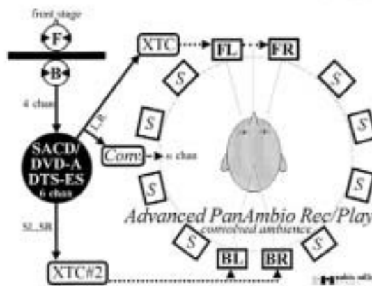
Fig. 6 Panorambiophonics Including Both Circular Direct Sound and Hall Ambience
