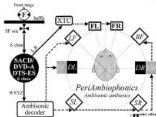
Fig. 8 Ambisonic Techniques Can Be Used to Provide Surround Ambience With Height
